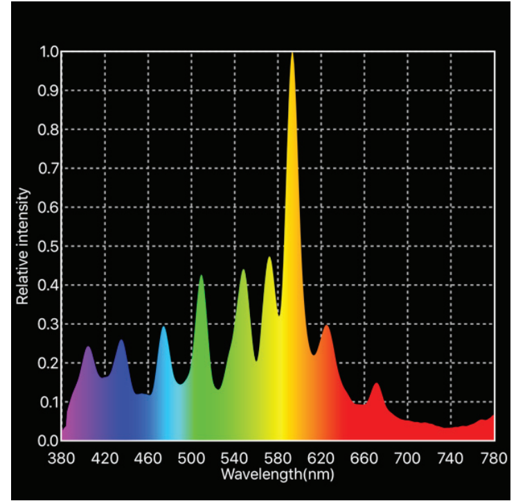
Spectrometer showing spectrum of light generated by the fixtures recently installed at Washington Park.
